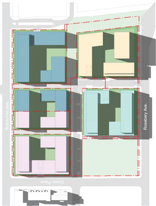
Shadow Diagram - DCP - March 22 3pm
